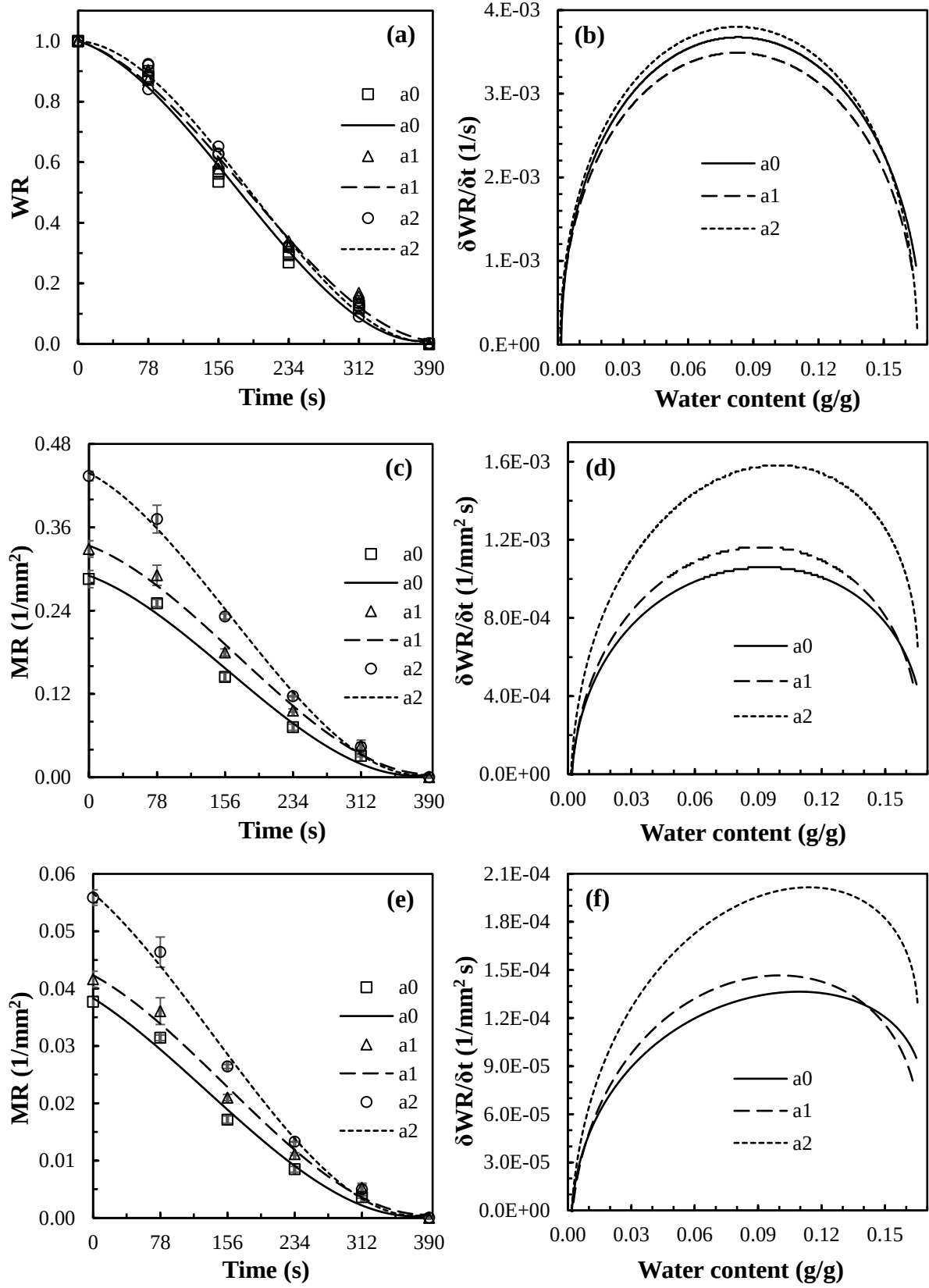
Figure 3. WR regression curves on a dry basis and their exchange profiles ( \delta WR / \delta t in absolute value) of floury (a0 and a1) and sweet (a2) maize kernels. Without kernel size approaches (a) and (b). Spatial (S/V) 2 approach (c) and (d). Distance (GMD/2) 2 approach (e) and (f). WR: water ratio. S: surface area, V: volume, and GMD: geometric mean diameter of individual maize kernels.
