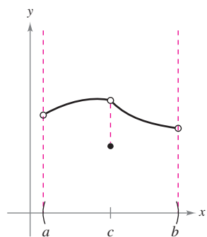
c) Discontinuidad evitable o removable Figura 1.26
